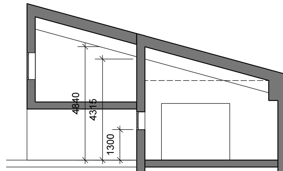
EXISTING SECTION
