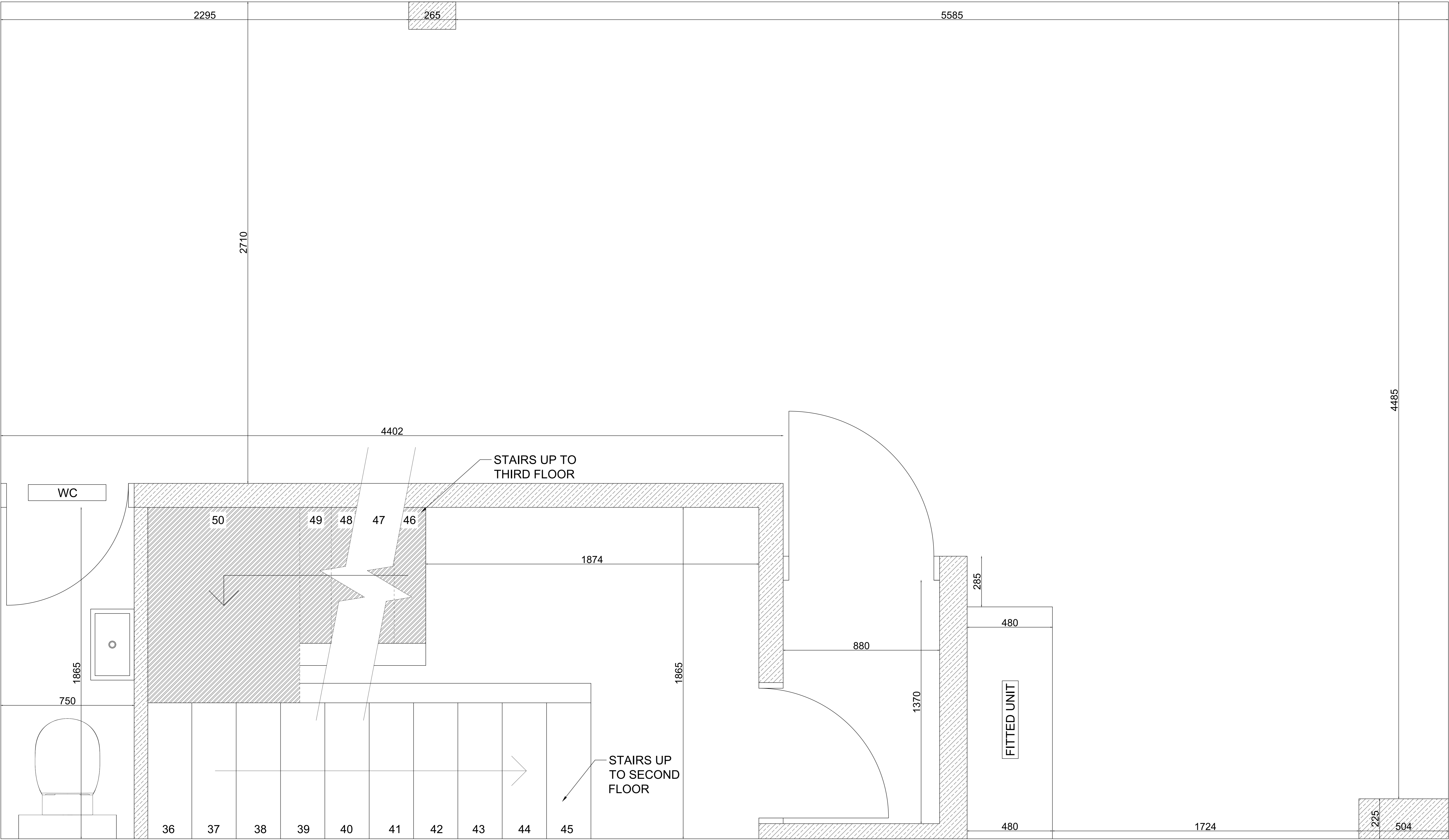
1 SECOND FLOOR PLAN Scale: 1:8
