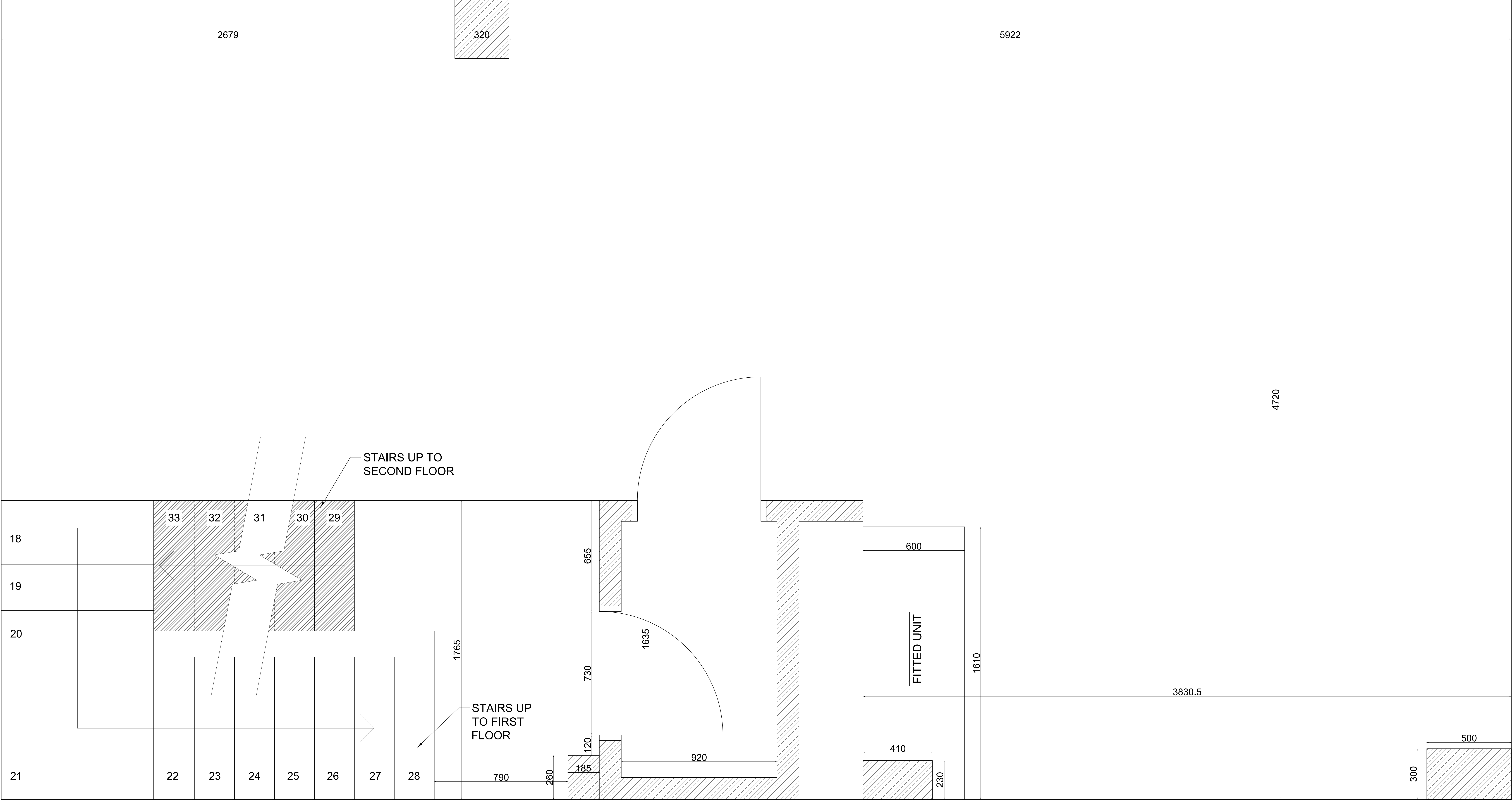
1 FIRST FLOOR PLAN Scale: 1:8
